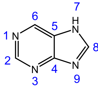
7H-Purin
