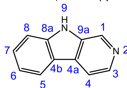
9H-β-Carbolin
