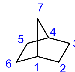
Bicyclo[2.2.1]heptan
