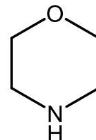
Morpholin
