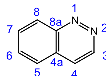
Cinnolin
