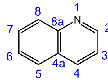
Chinolin (quinoline)
