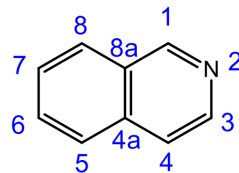
Isochinolin (isoquinoline)
