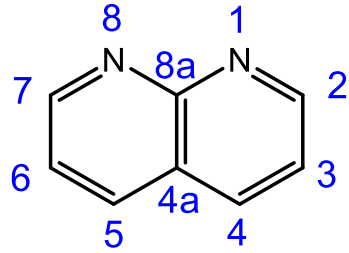
1,8-Naphthyridin
